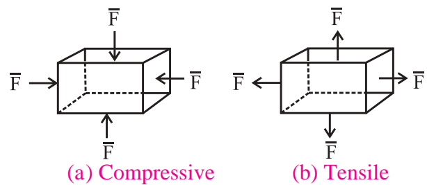
Fig. 2.2: Normal stress.
