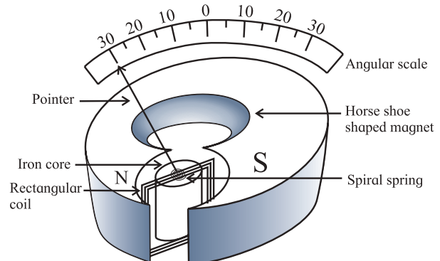
Fig. 9.12 Internal structure of galvanometer.
