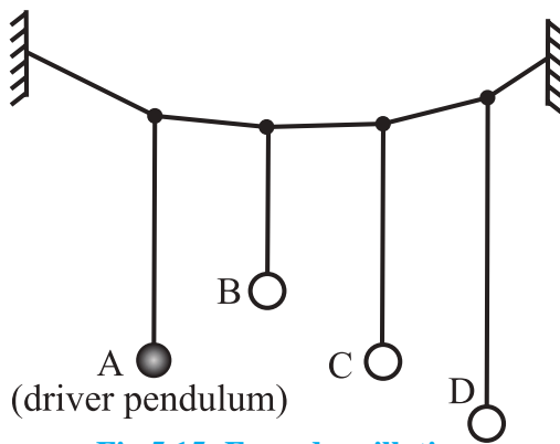
Fig 5.15: Forced oscillations.
