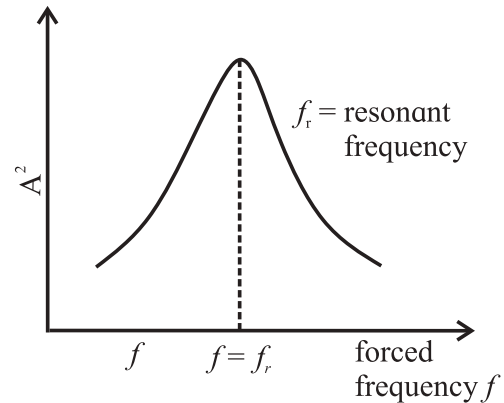
Fig 5.16: Resonant frequency.
