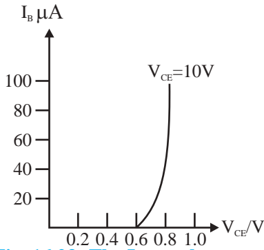
Fig. 16.23: The Input characteristics
