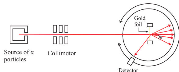
Fig.15.1: Geiger-Marsden experiment.
