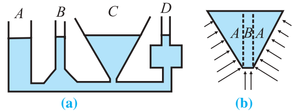
Fig. 2.10: Hydrostatic paradox.
