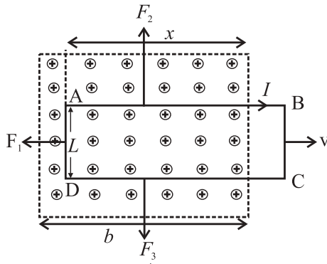
⊗ Magnetic field \vec{B} into plane of the paper
