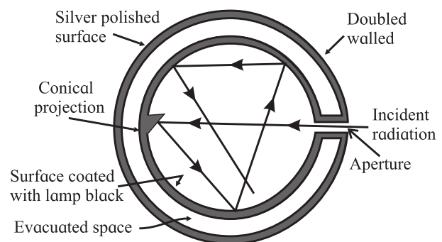
Fig. 3.4: Ferry's blackbody.
