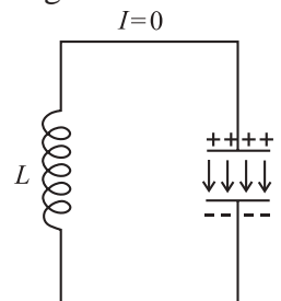
Fig. 13.16 (a) Let a capacitor with initial charge q_0 at (t = 0) be connected to an ideal inductor (zero resistance). The
