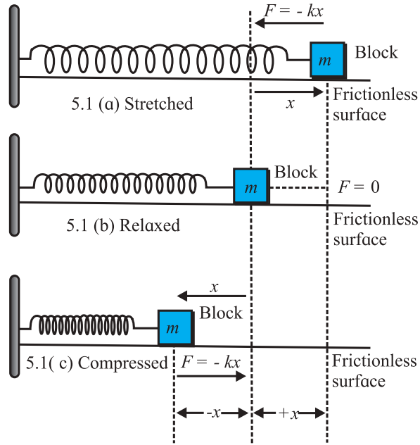
Fig. 5.1 (a), (b) and (c): Spring mass oscillator.
