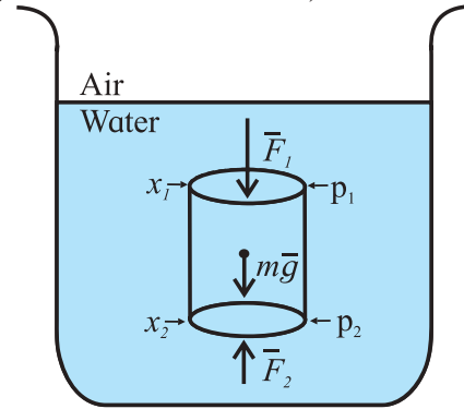
Fig. 2.7: Pressure due to an imaginary cylinder of fluid.
