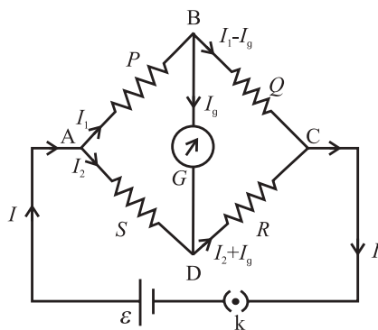
Fig. 9.4 : Wheatstone bridge.
