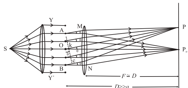
Fig. 7.14: Set up for fraunhofer diffraction .
