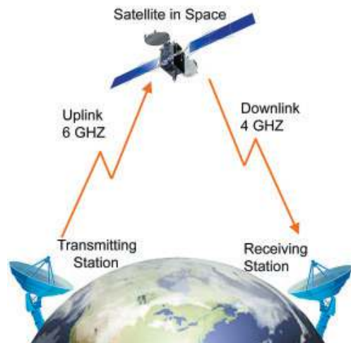
Fig. 8.14 : Satellite link
