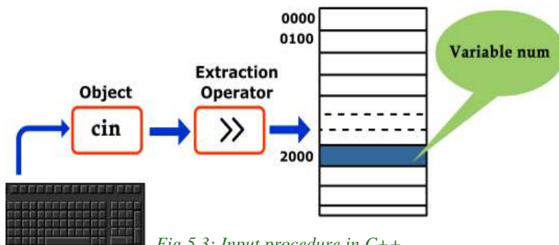
Fig 5.3: Input procedure in C++
