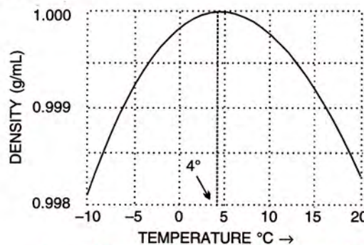
Fig. 3.3 Water has maximum density at 4°C
